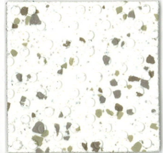
Cascade IPT20809
