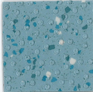
Rainfall IPT20810
