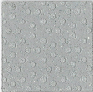
Gull T20813
