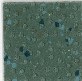
Fen IPT20815
