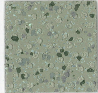
Seagrass IPT20814
