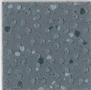
Shark IPT20812
